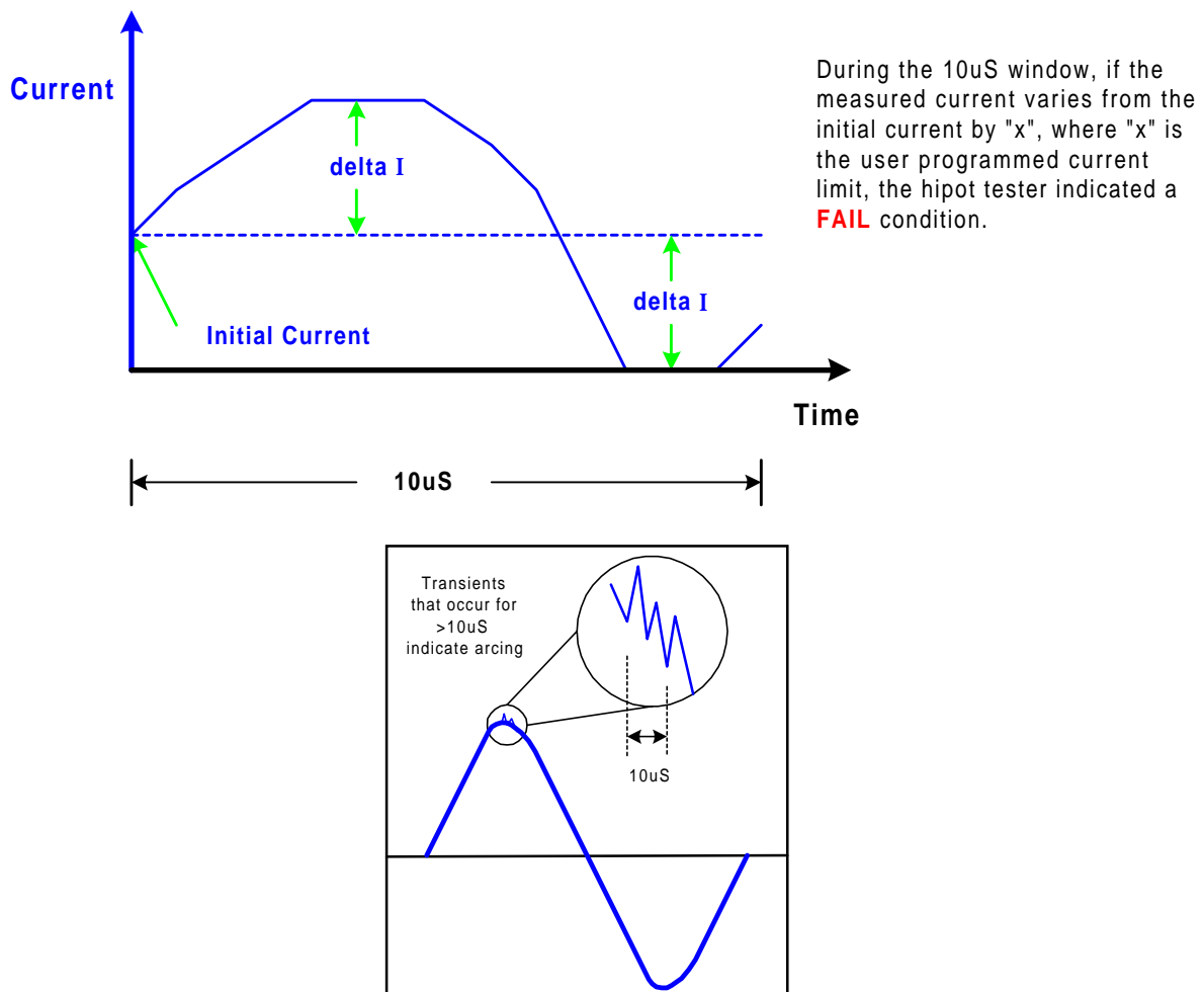
Figure 3: Arc Detection
